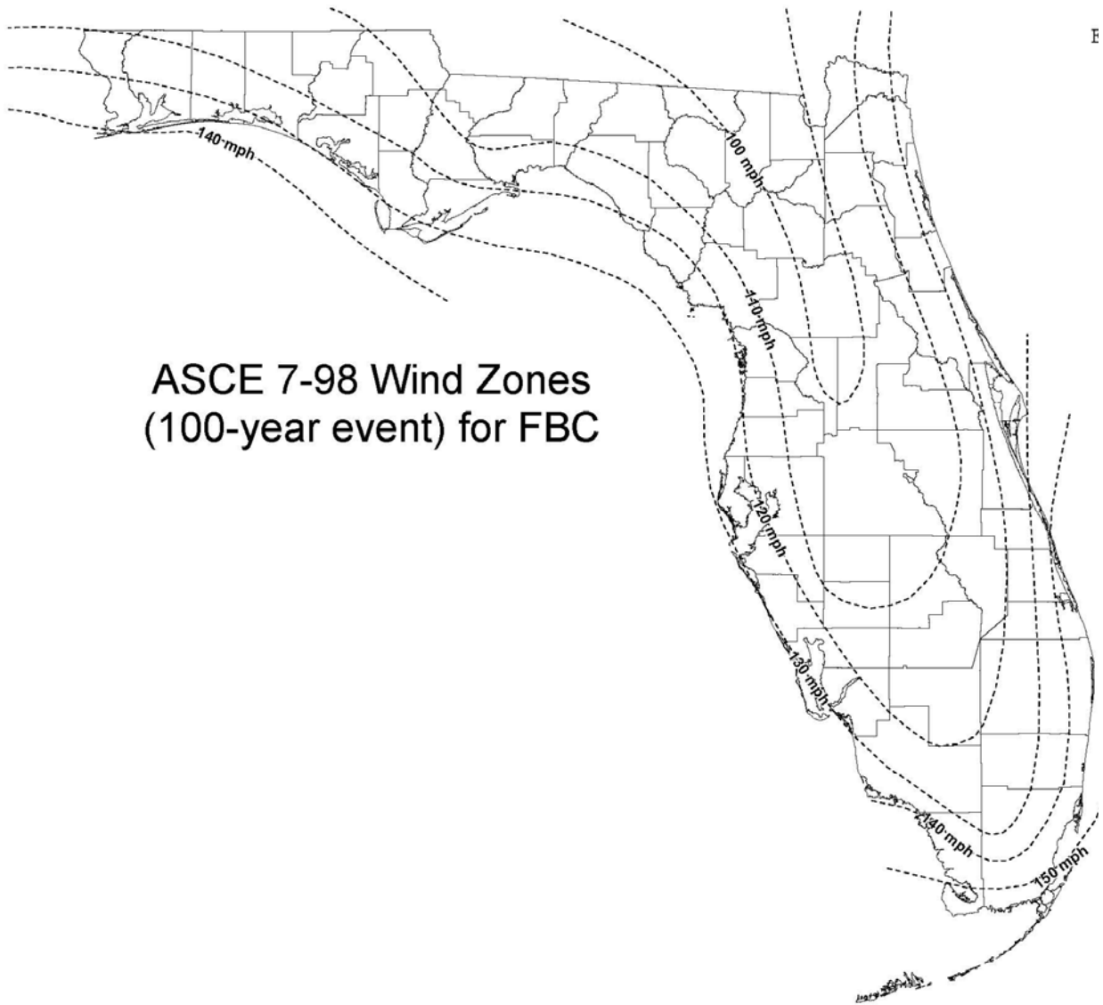
Figure II-7 ASCE 7-98 Wind Zones
